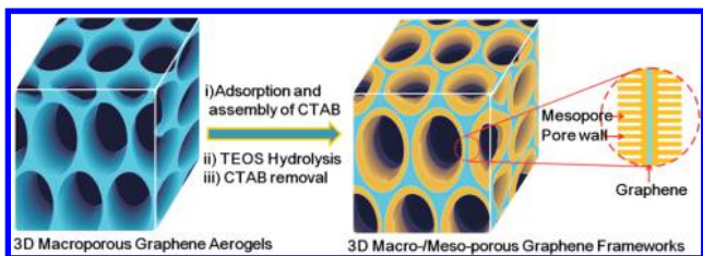
Figure 1. Fabrication of hierarchical macro- and mesoporous GA-SiO 2 frameworks: (i) electrostatic adsorption and assembly of CTAB on the surface of 3D GAs, (ii) TEOS hydrolysis for nucleation and growth of mesoporous silica on the surface of CTA + -adsorbed GAs, and (iii) CTAB removal through ethanol washing, drying, and thermal annealing.
